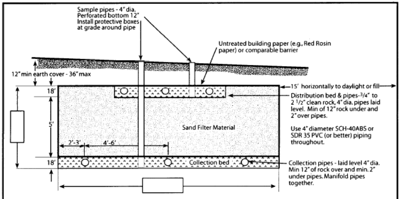
Cross Section
